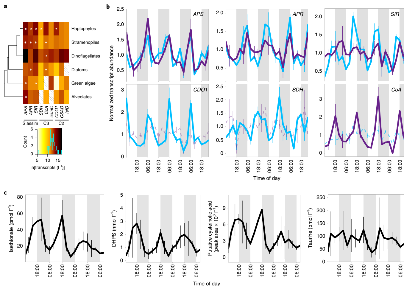
Fig. 2 | Daily sulfonate dynamics over a 4-d period in the North Pacific Subtropical Gyre. a , ln mean transcript abundances per litre of seawater over 4 d ( n=48 ) for sulfate assimilation (S assim) and sulfonate biosynthesis (C 2 and C 3 ) gene homologues in major eukaryotic phytoplankton taxa. The asterisks denote those genes with statistically significant diel periodicity based on the RAIN package 69 with the false discovery rate Bonferroni correction method ( P < 0.05 ). The dotted lines indicate that the gene homologue is not present in the taxon. Diatoms and dinoflagellates were analysed separately and thus are not included in the denoted stramenopile and alveolate groups. The legend shows the ln transcript abundance colour code and gene counts by transcript abundance bin. b , Mean transcript abundance of sulfate assimilation and sulfonate metabolism gene homologues in haptophytes (blue) and stramenopiles (purple) per time point ( n=2 ) versus transcript mean over the course of the diel study ( n=48 ). Those transcripts that showed statistically significant periodicity are in bold; those transcripts that were not significant are shown with dashed lines. The error bars represent the range of biological duplicates ( n=2 ). c , Mean sulfonate abundances in North Pacific Subtropical Gyre plankton that showed statistically significant diel periodicity based on the RAIN package 69 with the false discovery rate Bonferroni correction method ( P < 0.05 ) over the course of the diel study. The error bars represent the standard deviation of biological triplicates ( n=3 ).
