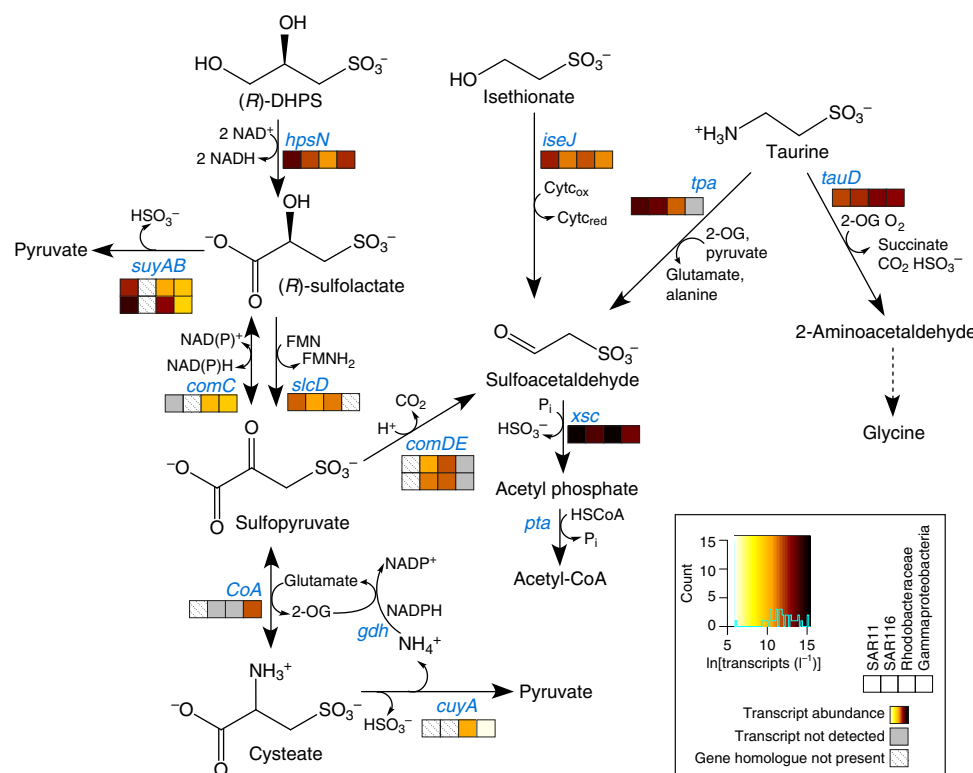
Fig. 3 | C 2 -sulfonate and C 3 -sulfonate catabolism by heterotrophic bacteria in the North Pacific Subtropical Gyre. Mean transcript inventories per litre of seawater ( n = 2 ) for gene homologues (blue) in major heterotrophic prokaryotic taxa. The legend shows the ln transcript abundance colour code and the gene counts by transcript abundance bin. Gene homologues that are present in the taxon but for which no transcripts were detected are shown in grey. Enzyme names for corresponding genes are as follows: comDE , sulfopyruvate decarboxylase; gdh , glutamate dehydrogenase; hpsN , DHPS 3-dehydrogenase; iseJ , isethionate dehydrogenase; pta , phosphate acetyltransferase; slcD , sulfolactate dehydrogenase; suyAB , sulfolactate sulfolase; tauD , taurine dioxygenase; cuyA , L-cysteate sulfolase. CoA, coenzyme A; CytC, cytochrome c; FMN, flavin mononucleotide.
